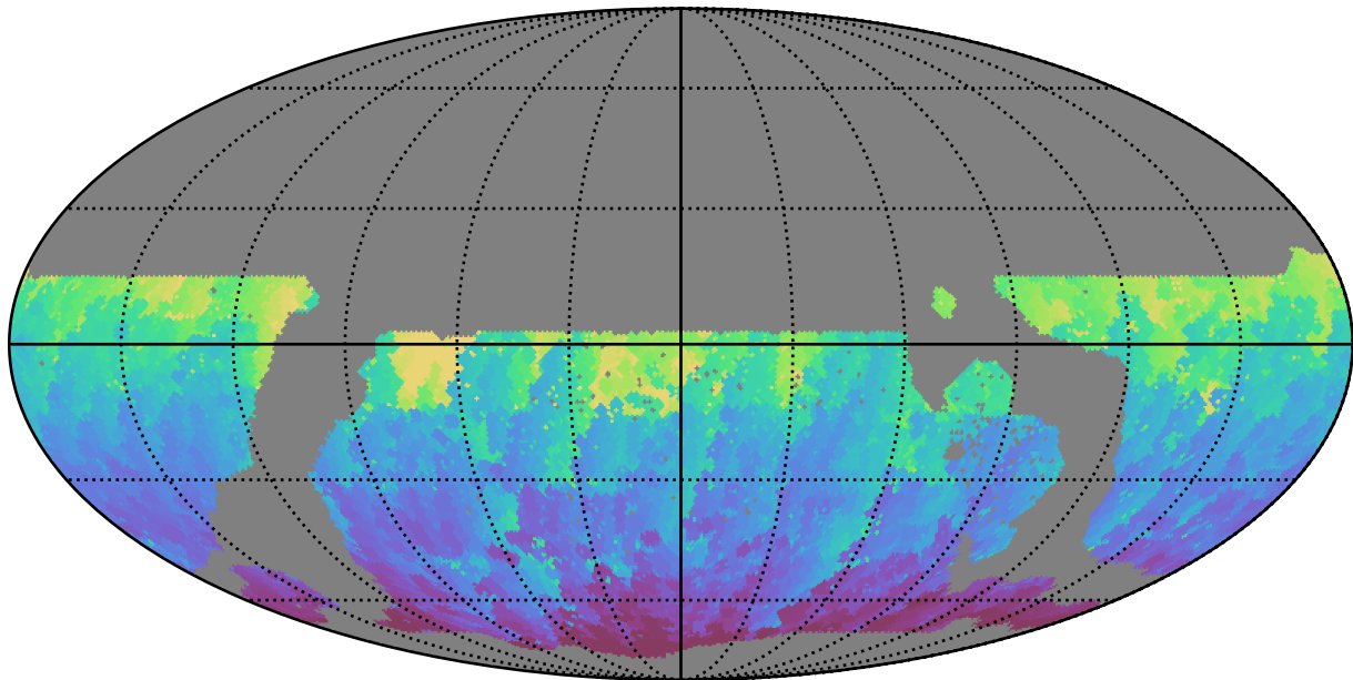
ddf_loaded_half_f12_v3.4_10yrs WFD g band: Min HA
