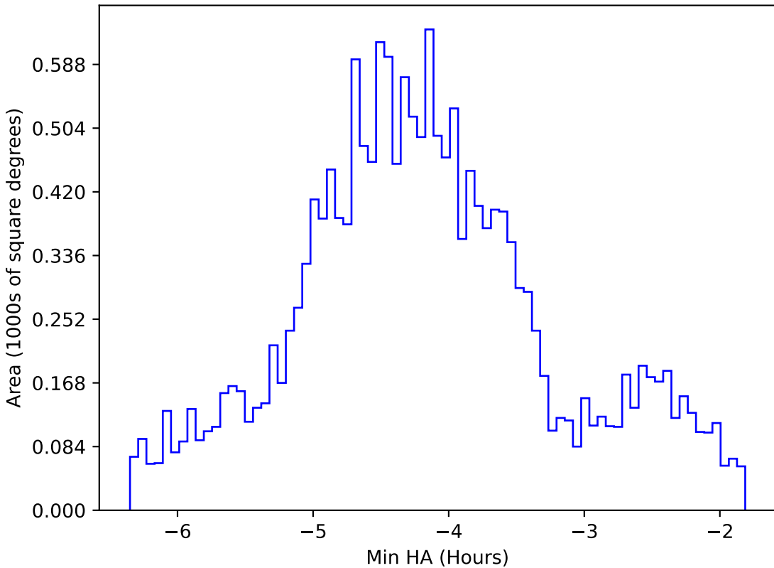
ddf_loaded_half_fl2_v3.4_10yrs WFD g band: Min HA
