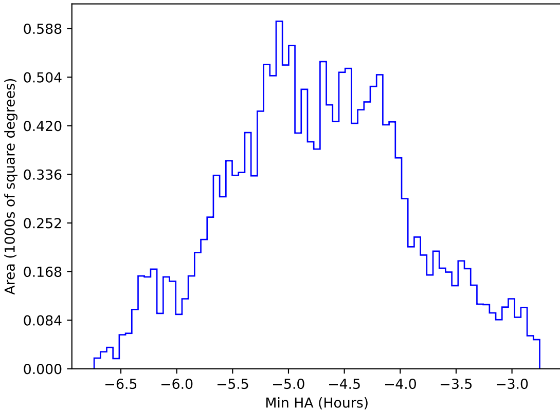
ddf_loaded_half_fl2_v3.4_10yrs WFD all bands: Min HA
