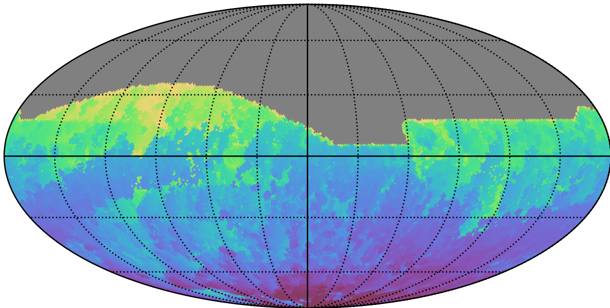
ddf_loaded_half_fl2_v3.4_10yrs All sky z band: Min HA
