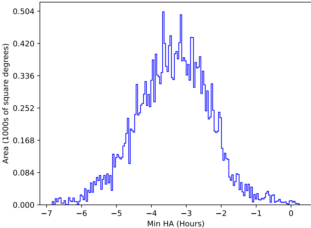
ddf_loaded_half_fl2_v3.4_10yrs All sky y band: Min HA
