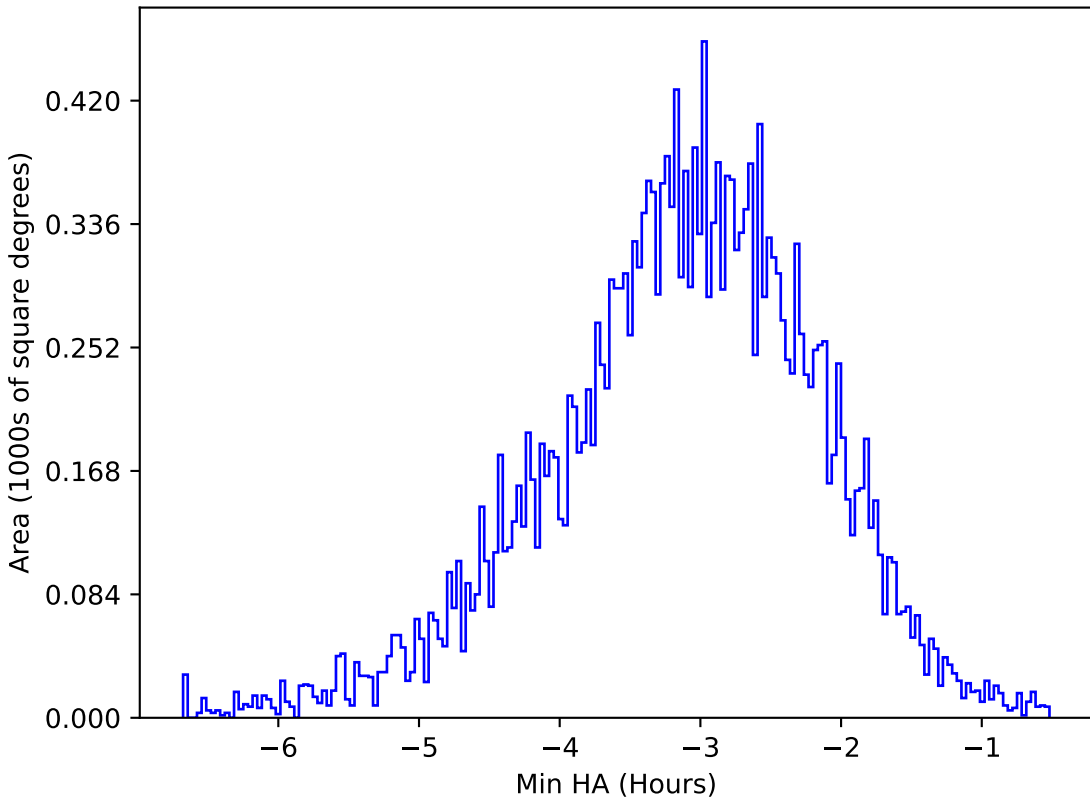
ddf_loaded_half_fl2_v3.4_10yrs All sky u band: Min HA
