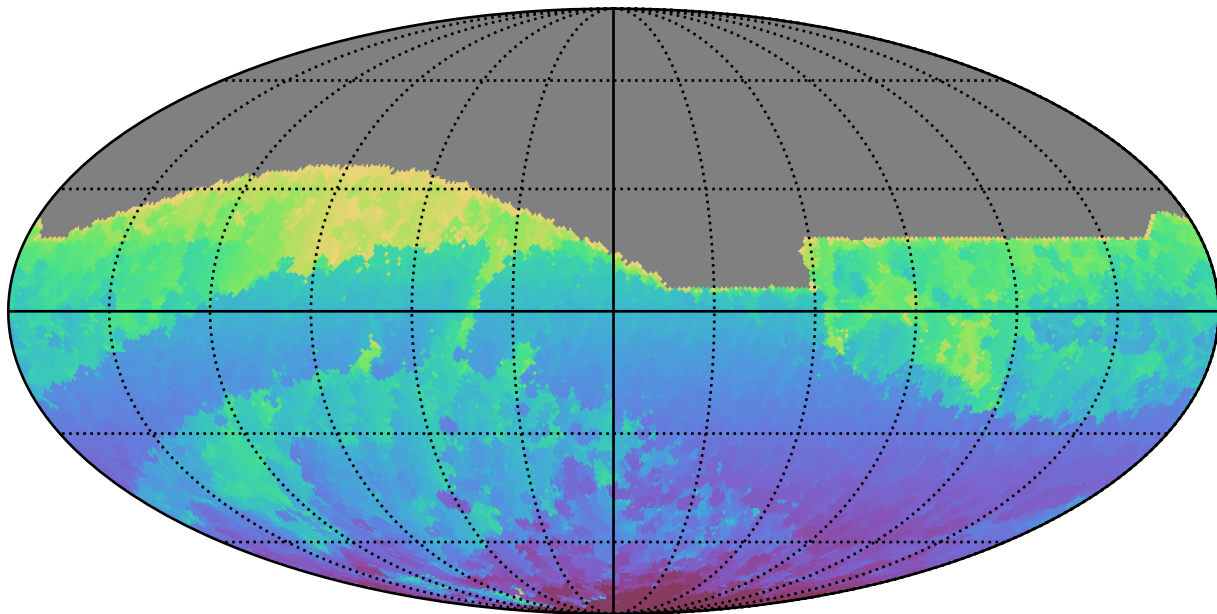
ddf_loaded_half_fl2_v3.4_10yrs All sky r band: Min HA
