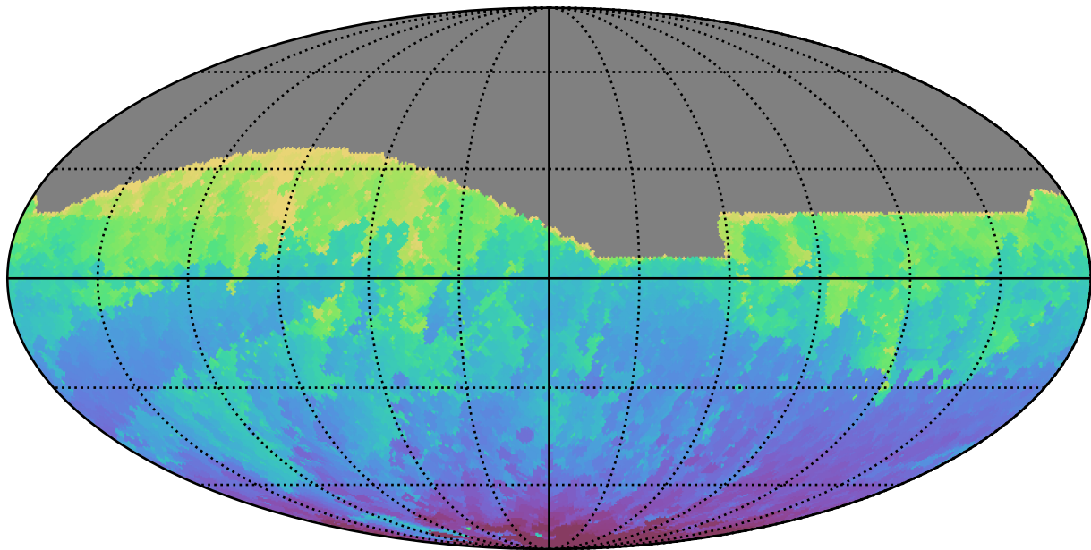
ddf_loaded_half_fl2_v3.4_10yrs All sky i band: Min HA
