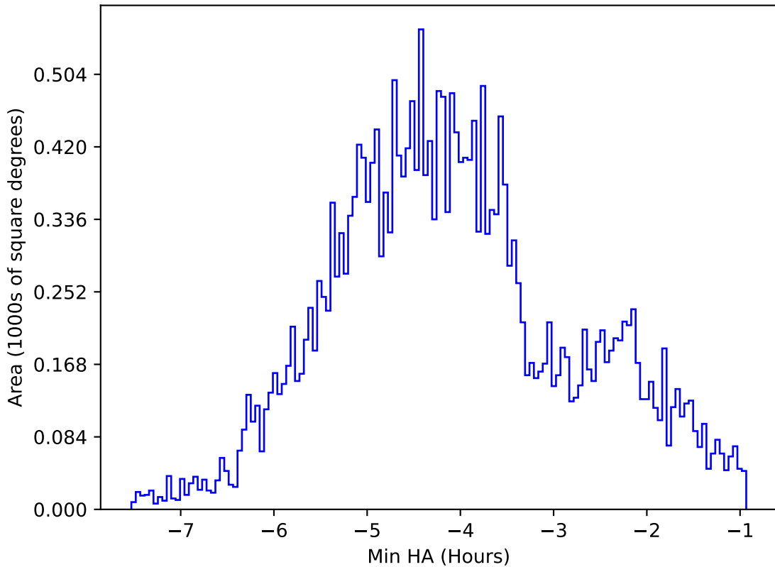
ddf_loaded_half_fl2_v3.4_10yrs All sky i band: Min HA
