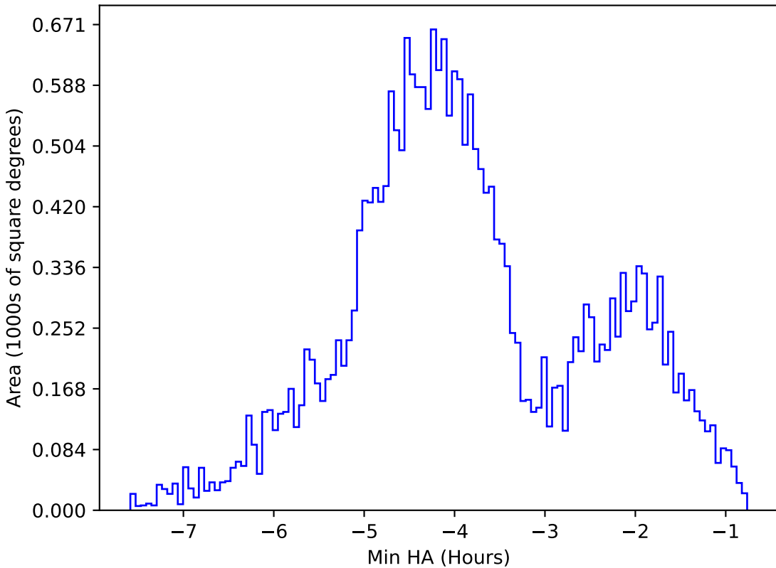
ddf_loaded_half_fl2_v3.4_10yrs All sky g band: Min HA
