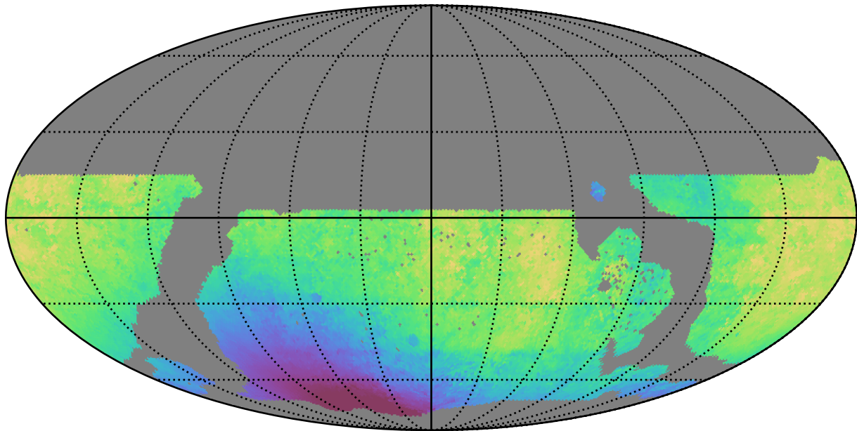
ddf_loaded_half_fl2_v3.4_10yrs WFD y band: Median solarElong
