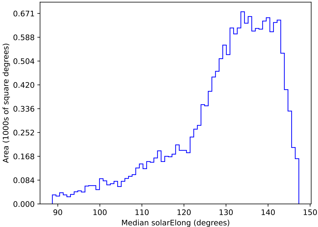
ddf_loaded_half_fl2_v3.4_10yrs WFD y band: Median solarElong
