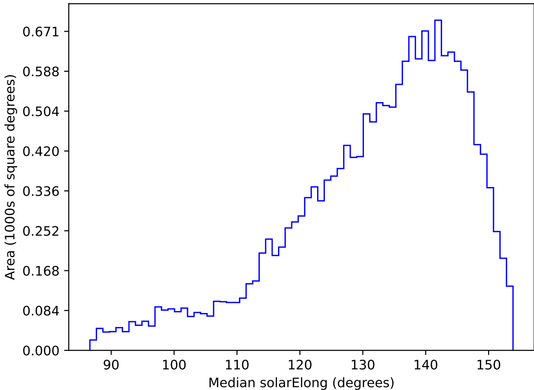
ddf_loaded_half_fl2_v3.4_10yrs WFD u band: Median solarElong
