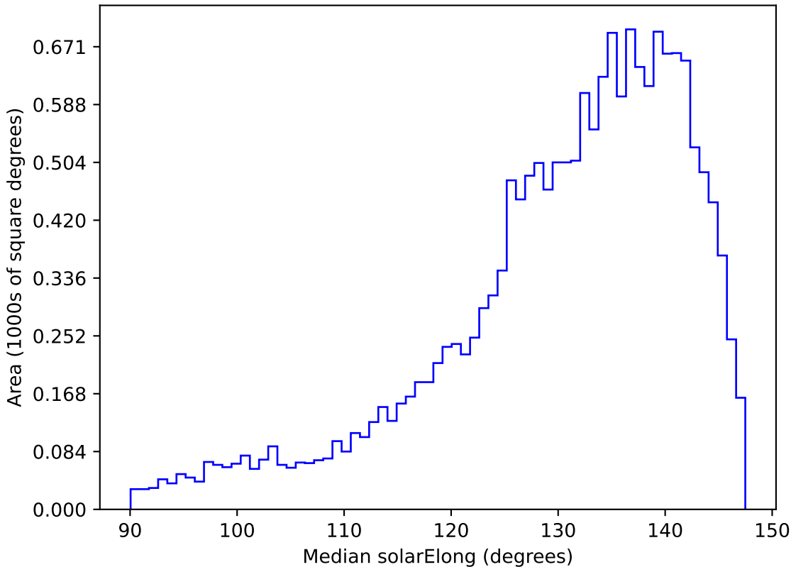
ddf_loaded_half_fl2_v3.4_10yrs WFD r band: Median solarElong
