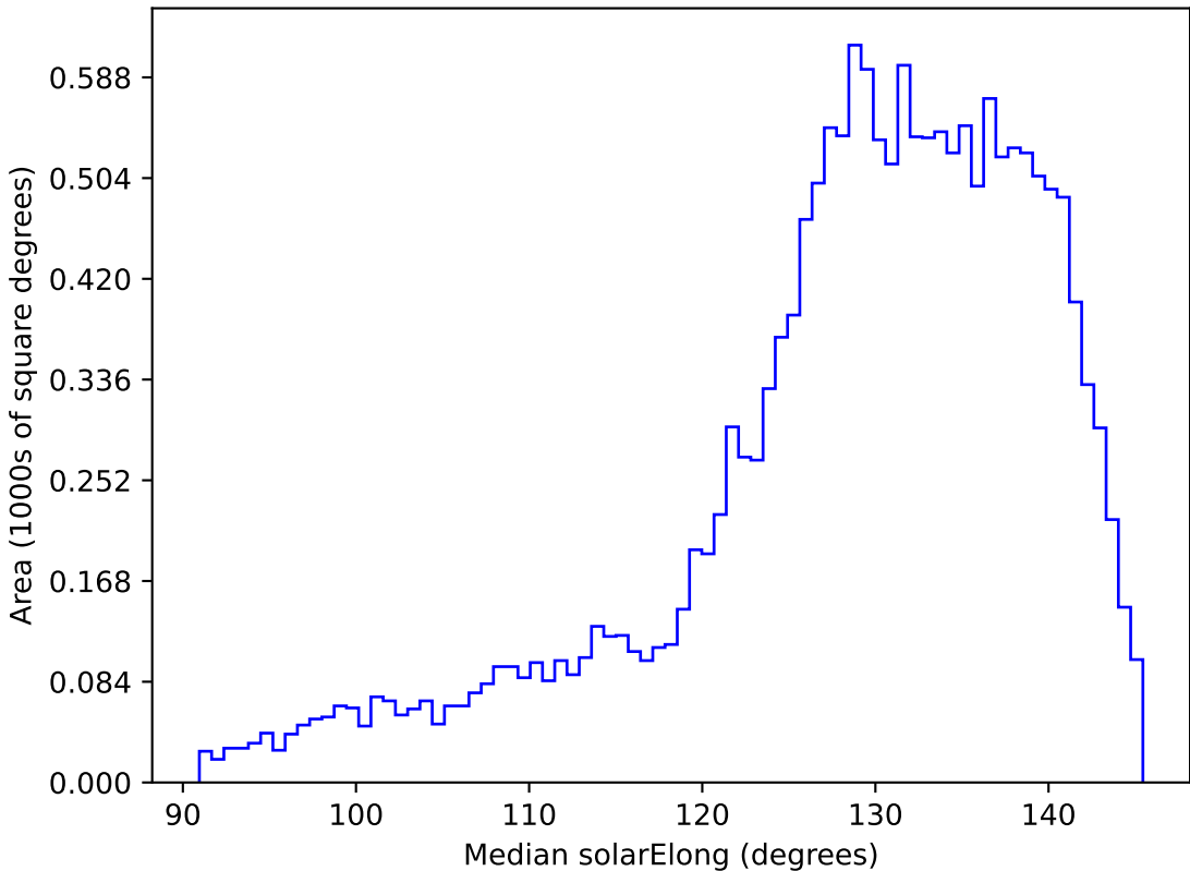
ddf_loaded_half_fl2_v3.4_10yrs WFD i band: Median solarElong
