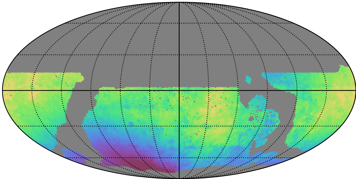
ddf_loaded_half_fl2_v3.4_10yrs WFD g band: Median solarElong
