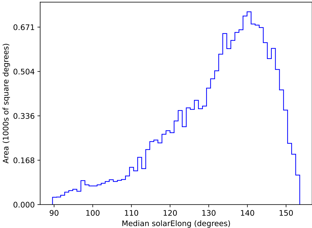
ddf_loaded_half_fl2_v3.4_10yrs WFD g band: Median solarElong
