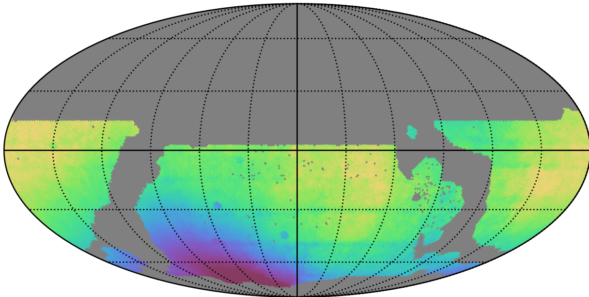
ddf_loaded_half_fl2_v3.4_10yrs WFD all bands: Median solarElong
