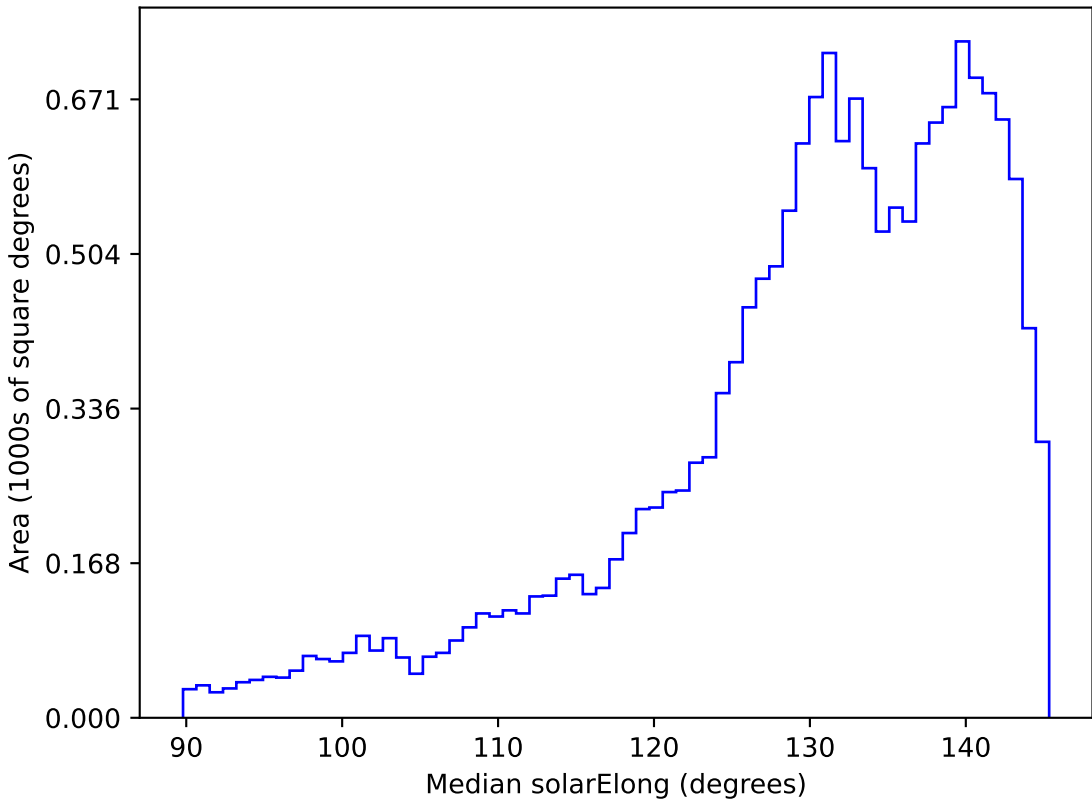
ddf_loaded_half_fl2_v3.4_10yrs WFD all bands: Median solarElong
