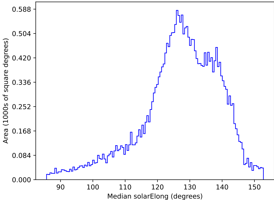
ddf_loaded_half_fl2_v3.4_10yrs All sky z band: Median solarElong
