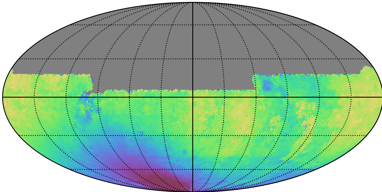
ddf_loaded_half_fl2_v3.4_10yrs All sky y band: Median solarElong
