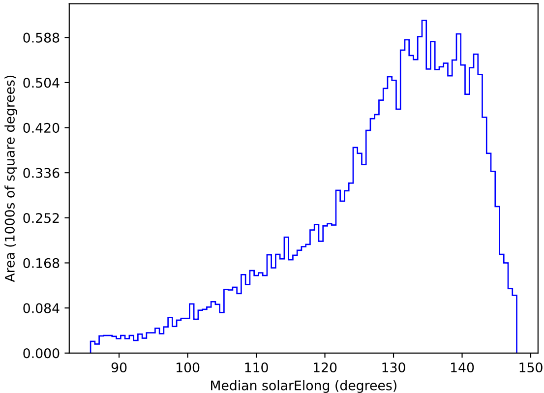
ddf_loaded_half_fl2_v3.4_10yrs All sky y band: Median solarElong
