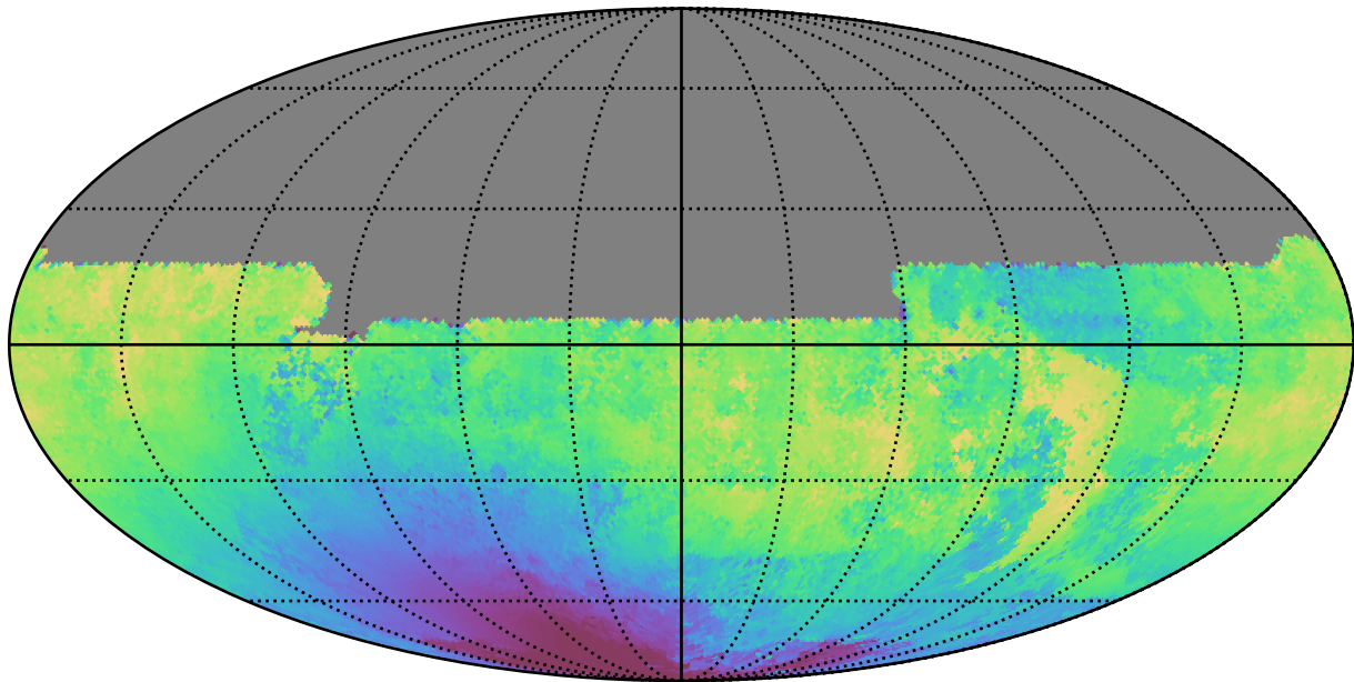
ddf_loaded_half_fl2_v3.4_10yrs All sky u band: Median solarElong
