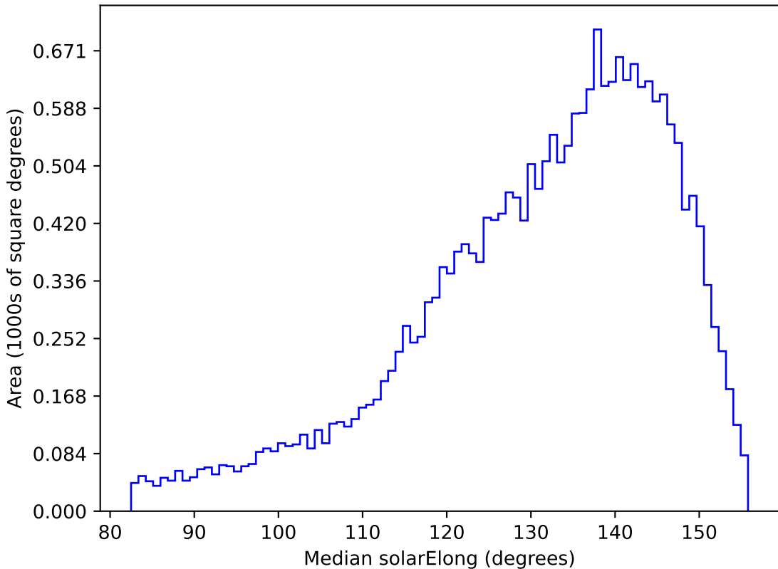
ddf_loaded_half_fl2_v3.4_10yrs All sky u band: Median solarElong
