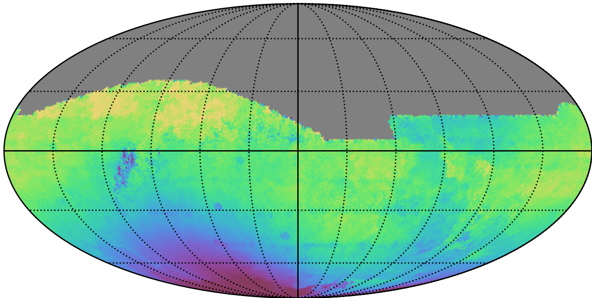
ddf_loaded_half_fl2_v3.4_10yrs All sky r band: Median solarElong
