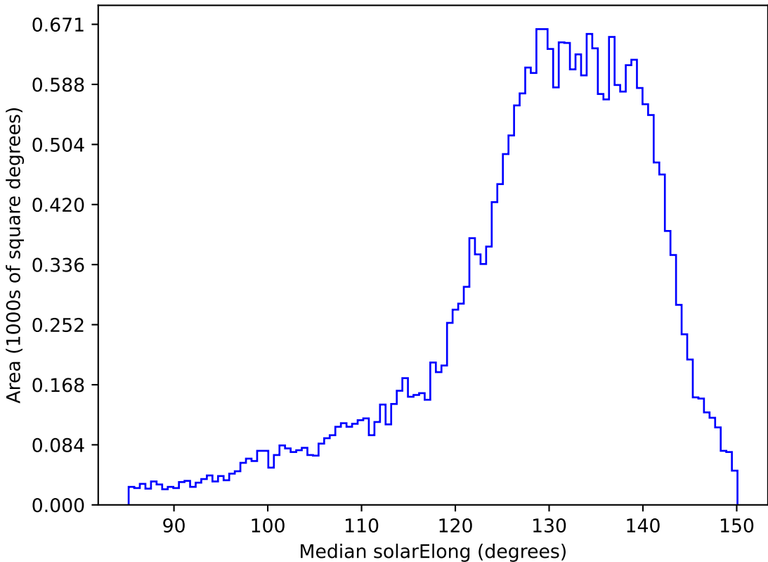
ddf_loaded_half_fl2_v3.4_10yrs All sky i band: Median solarElong
