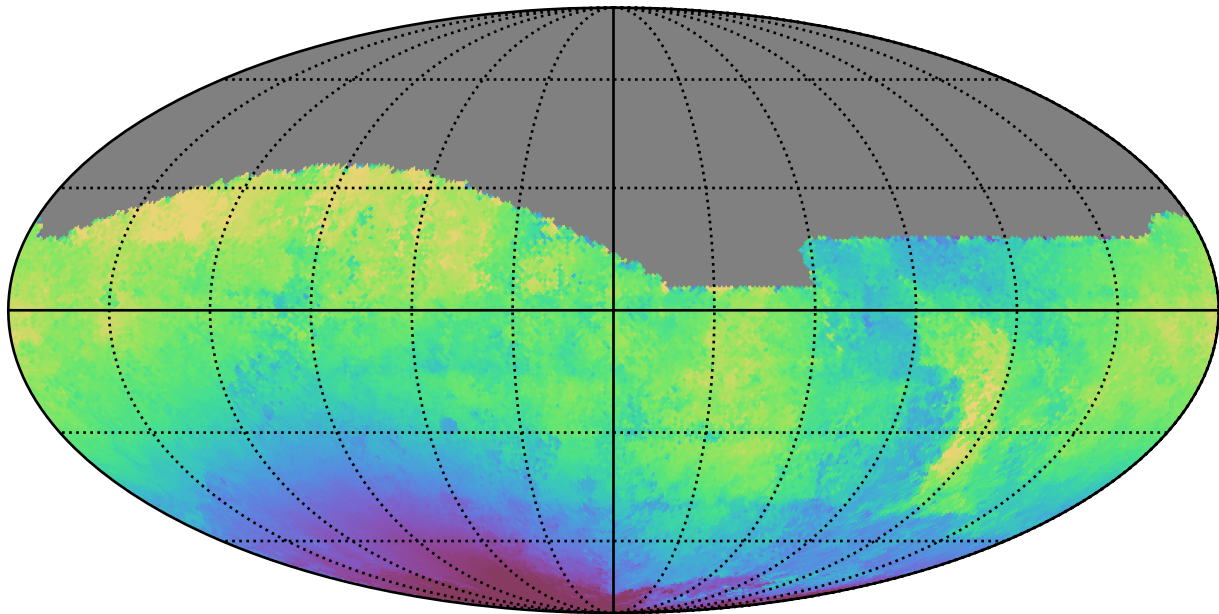
ddf_loaded_half_fl2_v3.4_10yrs All sky g band: Median solarElong
