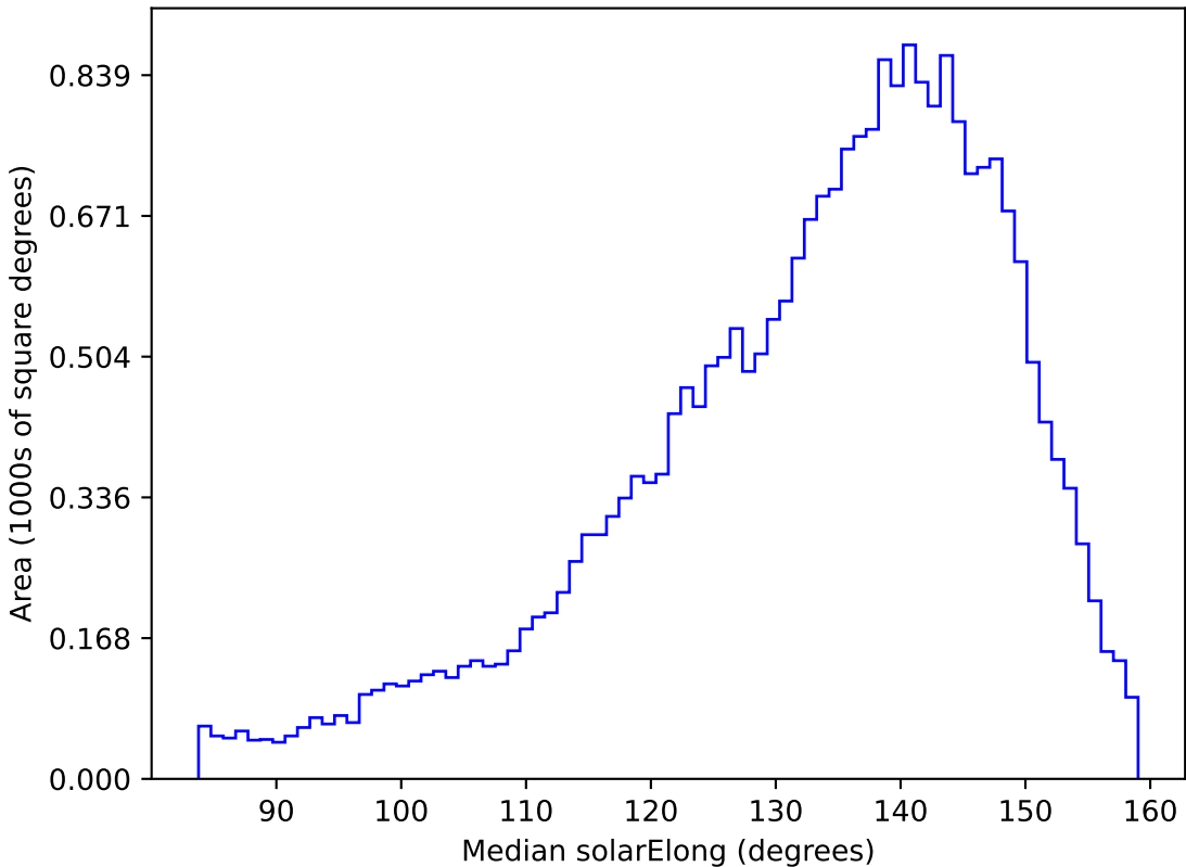
ddf_loaded_half_fl2_v3.4_10yrs All sky g band: Median solarElong
