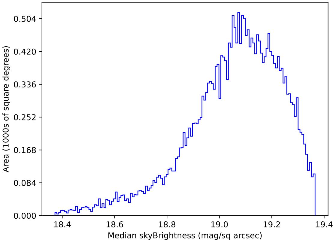
ddf_loaded_half_fl2_v3.4_10yrs Yr 1 z band: Median skyBrightness
