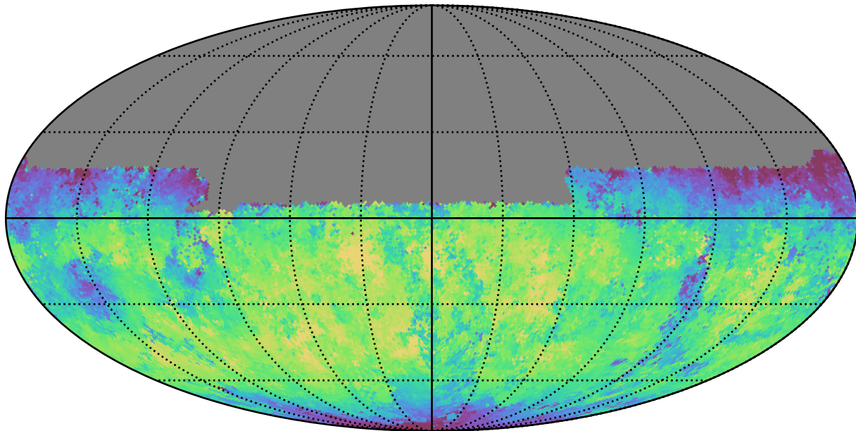
ddf_loaded_half_fl2_v3.4_10yrs Yr 1 y band: Median skyBrightness
