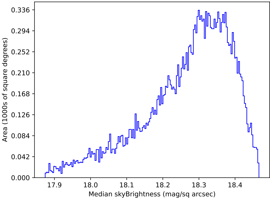
ddf_loaded_half_fl2_v3.4_10yrs Yr 1 y band: Median skyBrightness
