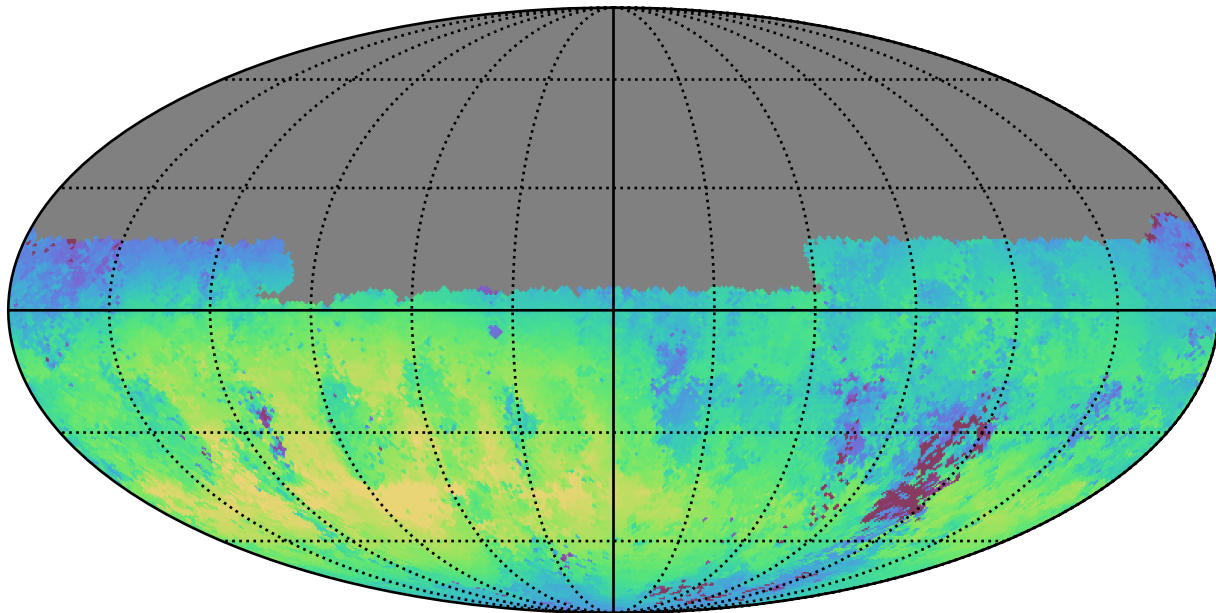
ddf_loaded_half_fl2_v3.4_10yrs Yr 1 u band: Median skyBrightness
