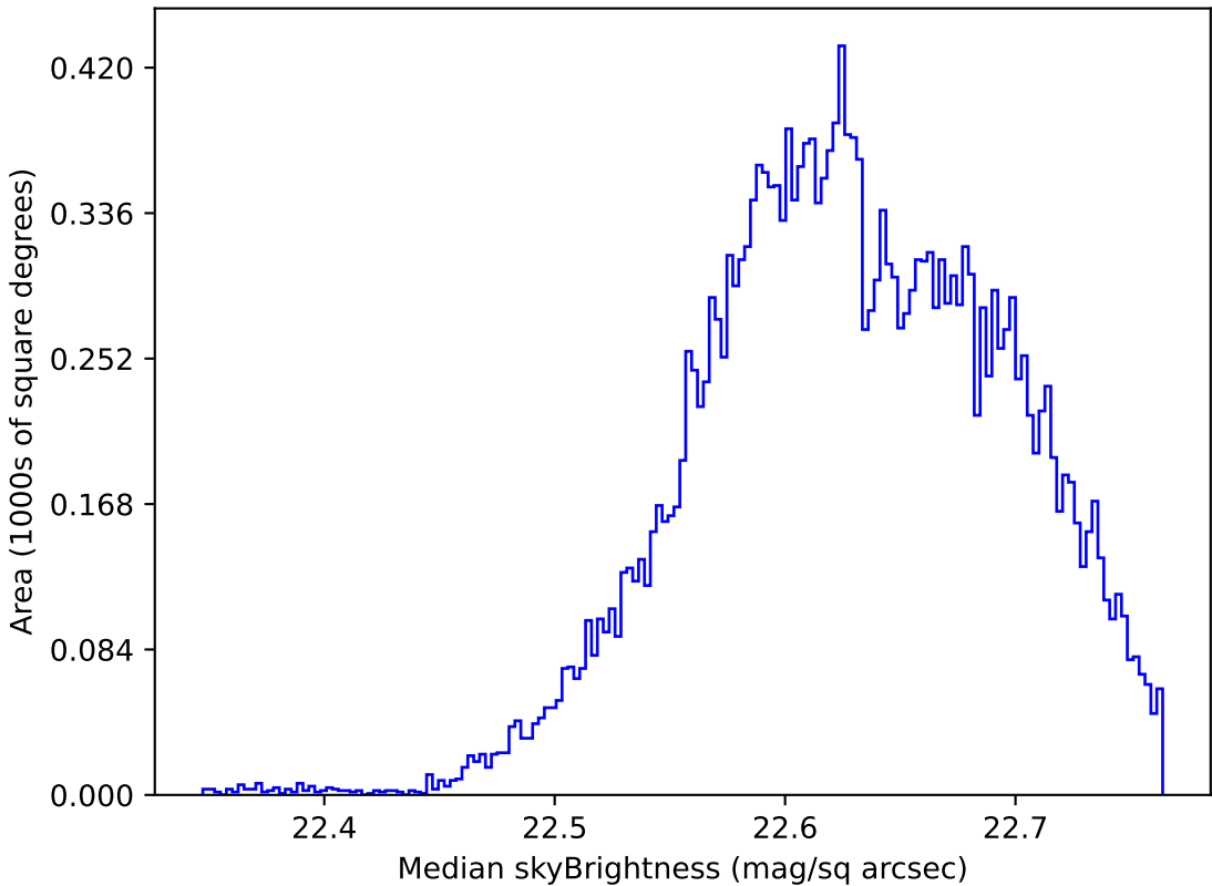
ddf_loaded_half_fl2_v3.4_10yrs Yr 1 u band: Median skyBrightness
