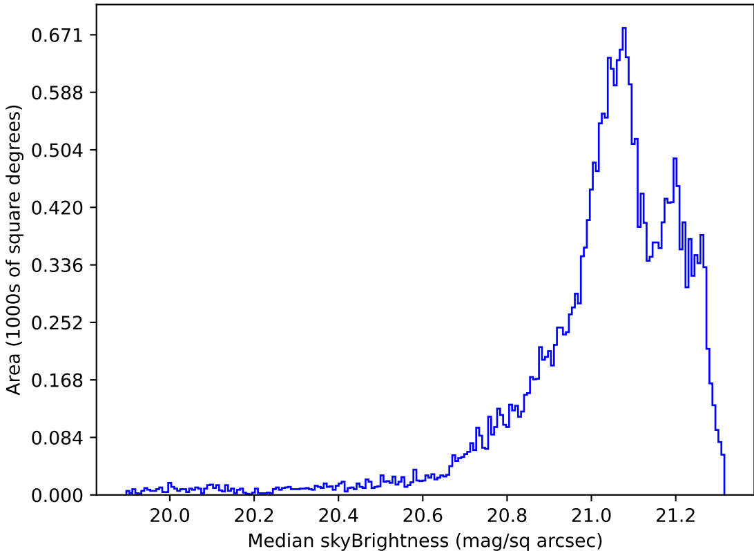
ddf_loaded_half_fl2_v3.4_10yrs Yr 1 r band: Median skyBrightness
