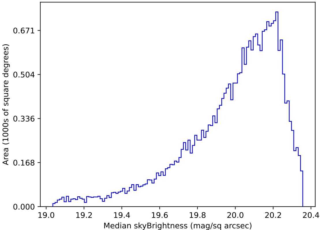
ddf_loaded_half_fl2_v3.4_10yrs Yr 1 i band: Median skyBrightness
