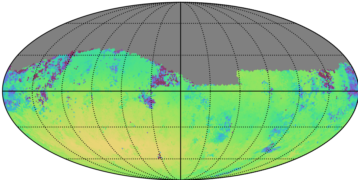
ddf_loaded_half_fl2_v3.4_10yrs Yr 1 g band: Median skyBrightness
