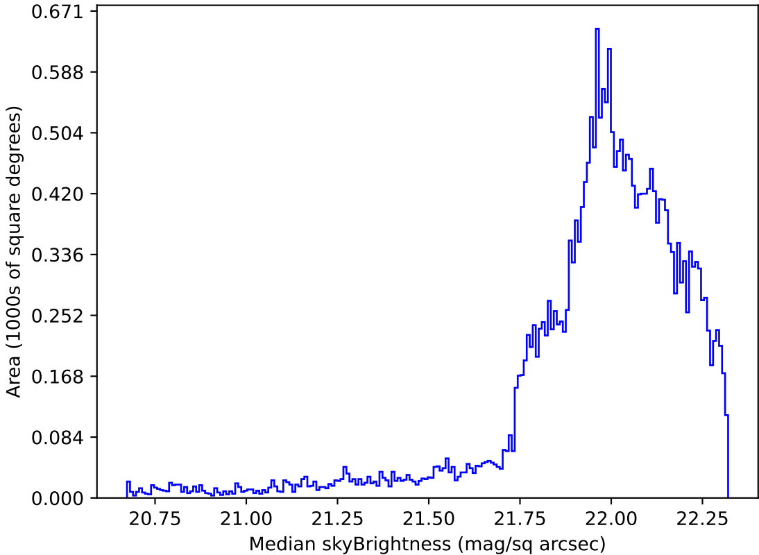
ddf_loaded_half_fl2_v3.4_10yrs Yr 1 g band: Median skyBrightness
