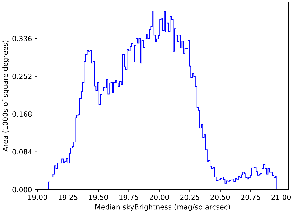
ddf_loaded_half_fl2_v3.4_10yrs Yr 1 all bands: Median skyBrightness
