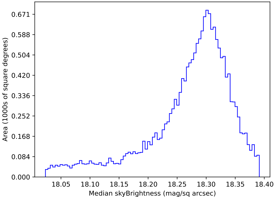
ddf_loaded_half_fl2_v3.4_10yrs WFD y band: Median skyBrightness
