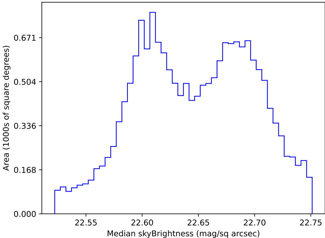
ddf_loaded_half_fl2_v3.4_10yrs WFD u band: Median skyBrightness
