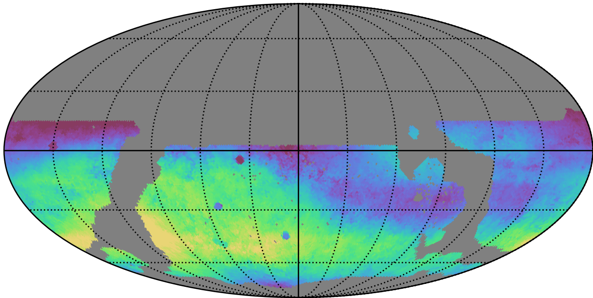
ddf_loaded_half_fl2_v3.4_10yrs WFD r band: Median skyBrightness
