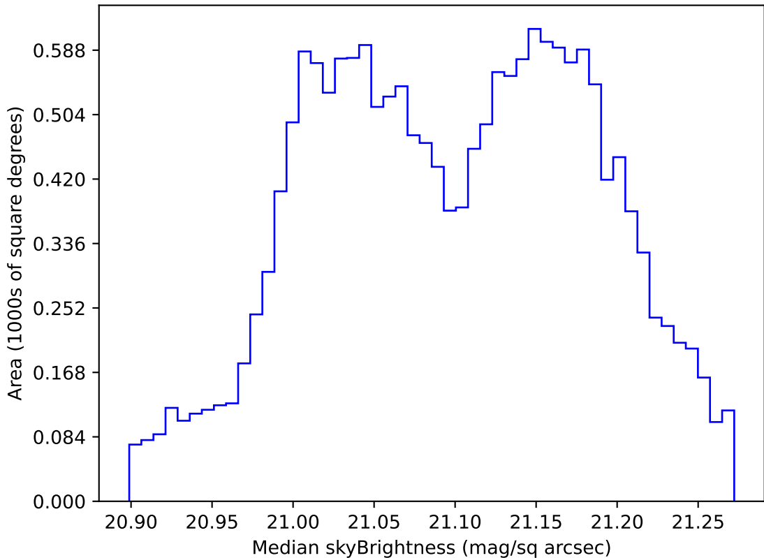
ddf_loaded_half_fl2_v3.4_10yrs WFD r band: Median skyBrightness
