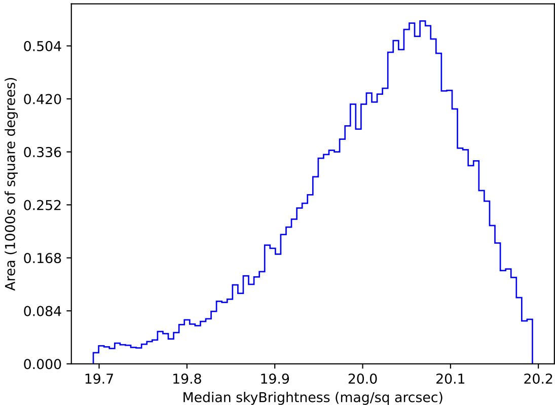
ddf_loaded_half_fl2_v3.4_10yrs WFD i band: Median skyBrightness
