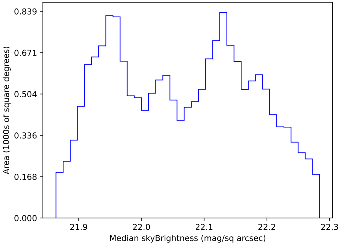
ddf_loaded_half_fl2_v3.4_10yrs WFD g band: Median skyBrightness
