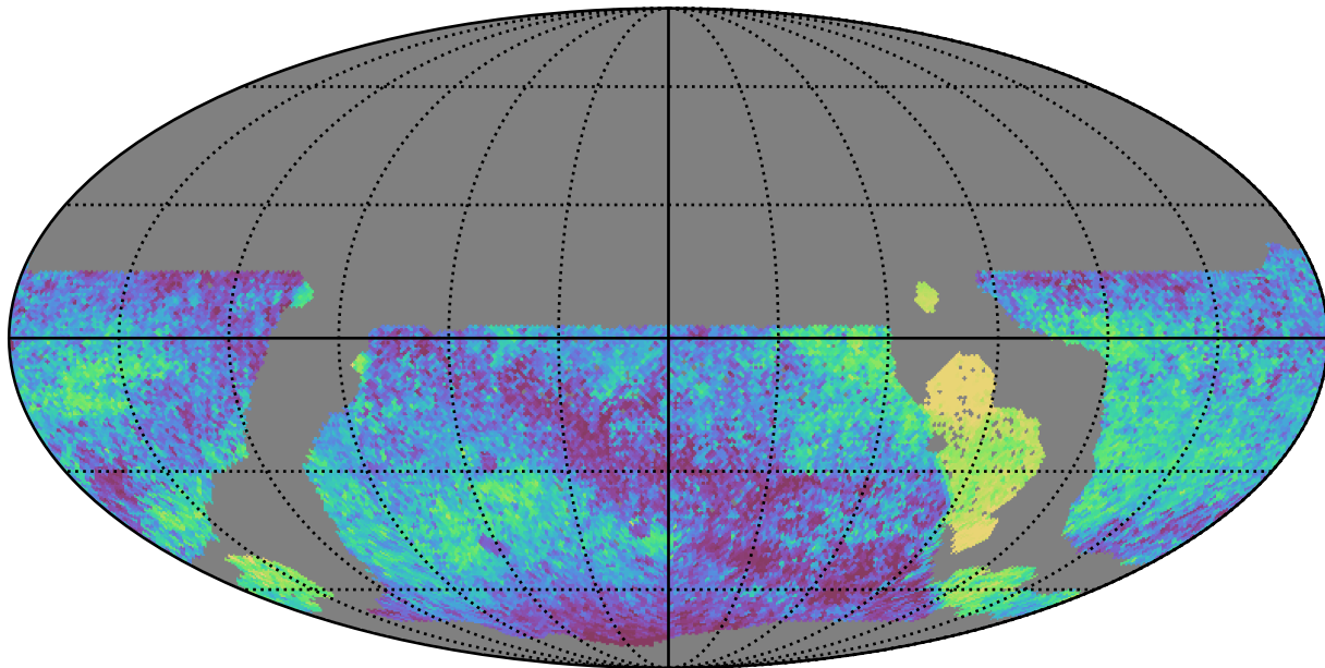
ddf_loaded_half_fl2_v3.4_10yrs WFD all bands: Median skyBrightness
