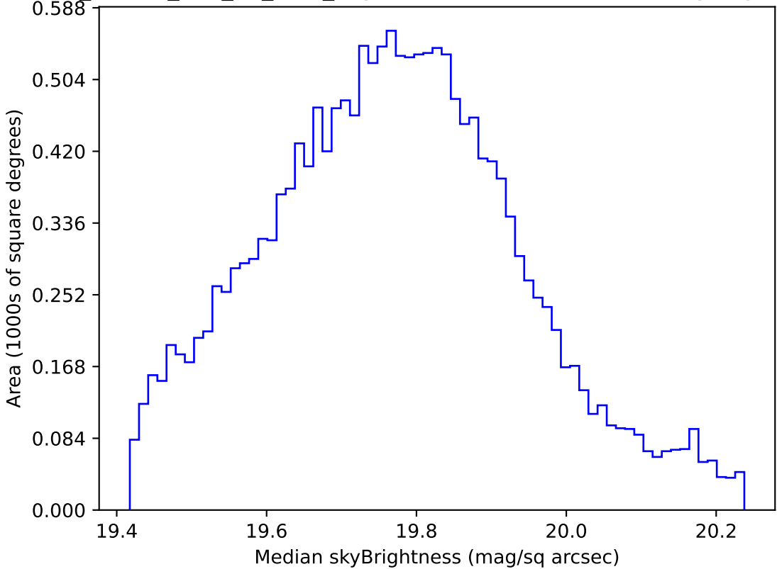
ddf_loaded_half_fl2_v3.4_10yrs WFD all bands: Median skyBrightness
