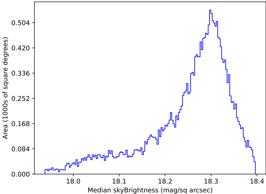
ddf_loaded_half_fl2_v3.4_10yrs All sky y band: Median skyBrightness
