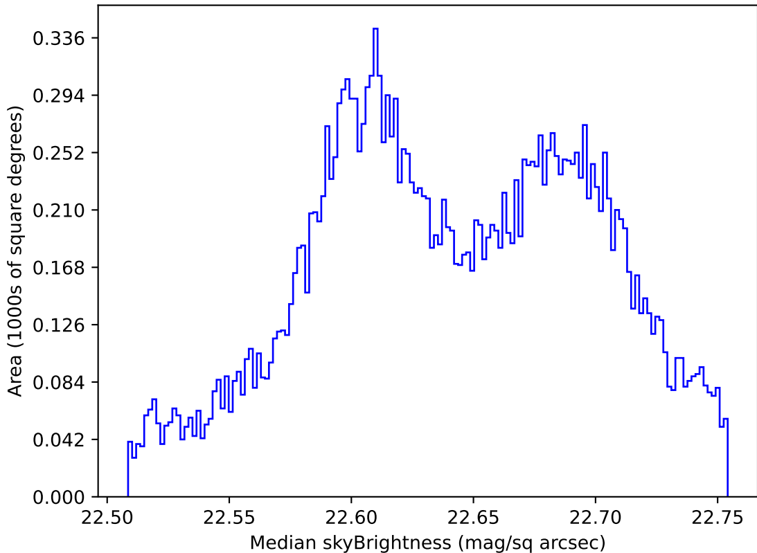
ddf_loaded_half_fl2_v3.4_10yrs All sky u band: Median skyBrightness
