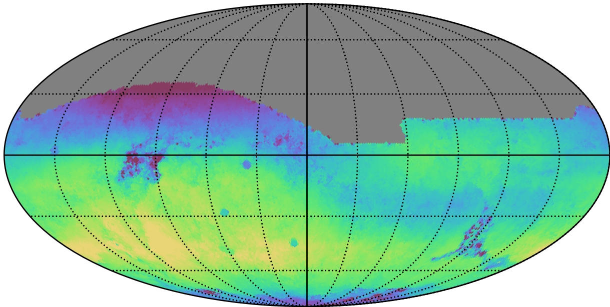
ddf_loaded_half_fl2_v3.4_10yrs All sky r band: Median skyBrightness
