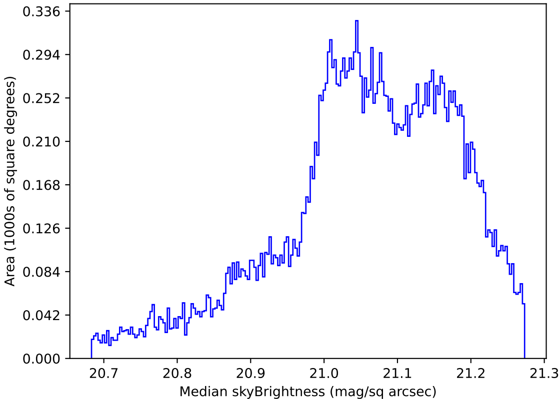
ddf_loaded_half_fl2_v3.4_10yrs All sky r band: Median skyBrightness
